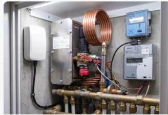
Compact (IP30)
